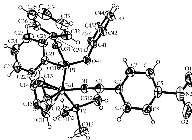
Figure 1 A view of the complex cation in (I), showing 30% probability displacement ellipsoids and the atomic labelling scheme.
